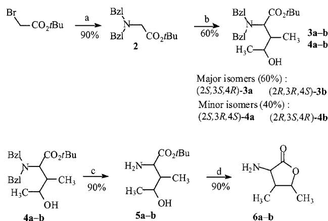
Scheme 1. Synthesis of (3 S ,4 R ,5 S )-3-amino-4,5-dimethyldihydrofuran-2-one ( 6a ) and (3 R ,4 S ,5 R )-3-amino-4,5-dimethyldihydrofuran-2-one ( 6b ): a) 2.2 mmol of dibenzylamine; b) 1) \text{LiHMDS} /THF (1 M, 1.5 mmol), 30 min, -30^\circ\text{C} ; 2) cis -2,3-dimethyloxirane (0.3 mmol/ \text{BF}_3 \cdot \text{Et}_2\text{O} /TMSCl); 3) \text{NH}_4\text{Cl} ; 4) diastereomers separation by silica gel column chromatography; c) \text{Pd}(\text{OH})_2/\text{C}/\text{MeOH} ; d) TFA (50% DCM)
