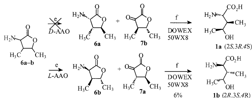
Scheme 2. Enzymatic enantioselective aminooxidation of 6a and 6b by D-AAO and L-AAO: e) phosphate buffer pH 8.3, \text{O}_2 bubbling, 1% \text{H}_2\text{O}_2 , catalase and D-AAO (or L-AAO), 1 day, RT; f) purification of mother solution liquor by DOWEX 50WX8 ion-exchange resin ( \text{H}^+ form)
